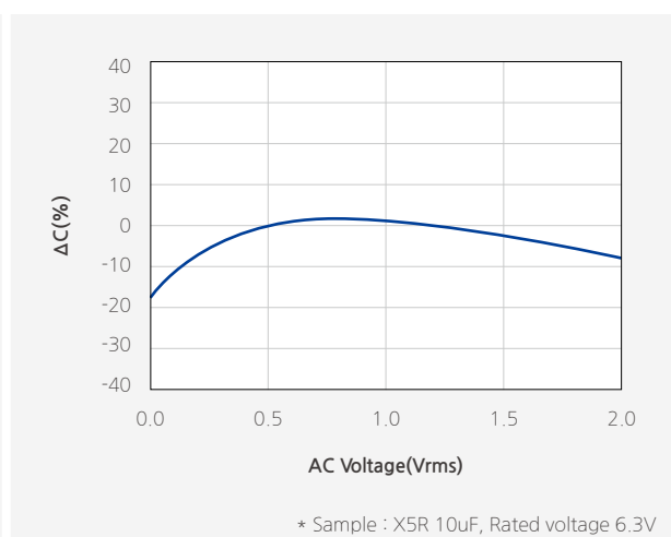
[Example of AC voltage characteristics]
