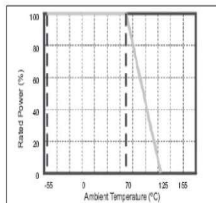
For Climatic category (IEC 60068) 55/125/56 (for 0201 type)
