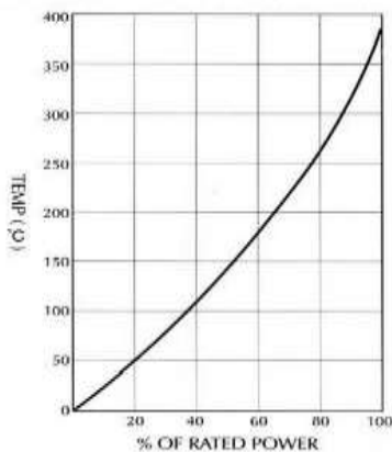
■ SURFACE TEMP. VS POWER LOAD
