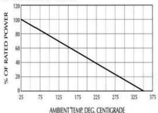
■ POWER RATING CHART
